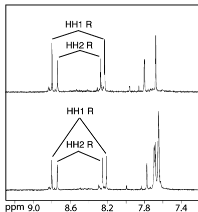
Figure 4. G* H8/T H6 region of 1D NMR spectra for ( R,S,S,R )-BipPt(d(G*G*T)) (top) and ( R,S,S,R )-BipPt(d(G*G*TTT)) (bottom) at equilibrium (pH \approx 4, 23 °C). Labels mark the G* H8 signals of the conformers. Most of the minor signals are from trace impurities; the signals at \sim 7.8 and 8.0 ppm are most likely from the \Delta HT1 conformer, but the amount of product was too small to characterize.
