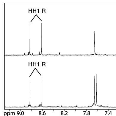
Figure 5. G* H8/T H6 region of 1D NMR spectra for ( R,S,S,R )-BipPt(d(TG*G*T)) (top) and ( R,S,S,R )-BipPt(d(TG*G*TT)) (bottom) at equilibrium (pH \approx 4, 23 °C). Labels mark the G* H8 signals of the conformers.
