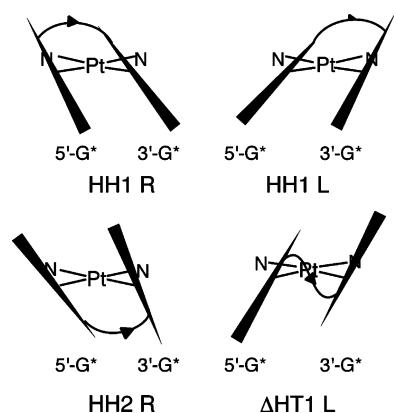
Figure 2. Schematic representation of right (R) and left (L) base canting for the Pt(d(G* p G*)) macrocyclic chelate ring of previously observed HH1, HH2, and ΔHT1 conformers. G* bases are shown as triangles, with the apex of the triangle representing the five-membered ring and the base of the triangle representing the six-membered ring.
