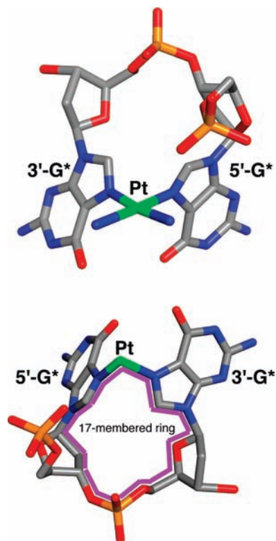
Figure 1. A representative structure of the Pt(G* p G*) cross-link. Top: Pt links adjacent G* residues to form the typical HH1 conformer. Bottom: A different view of the same molecule rotated to show the 17-membered chelate ring in an HH1 G*G* lesion and the anti conformation of the G* residues. The 17-membered ring is outlined in purple. These figures were generated by using molecule R1, one of the four cis -Pt(NH 3 ) 2 (d(pG* p G*)) structures characterized by X-ray crystallography. 12
