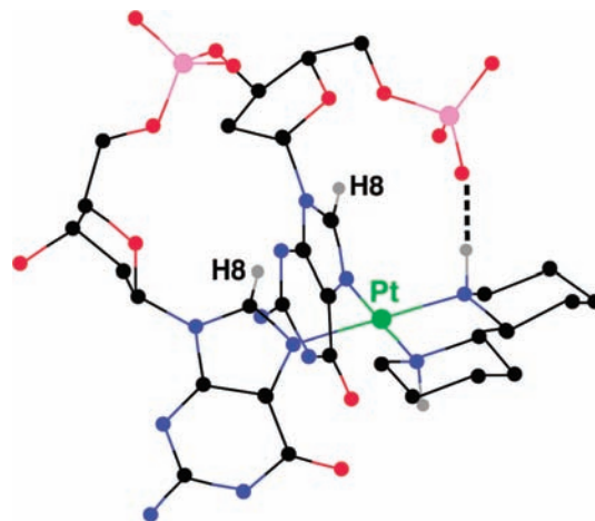
Figure 10. Ball-and-stick minimized MMD HH1 R model of (R,S,S,R)-BipPt(d(pG*pG*)). The dashed line indicates the H-bonding between the protonated 5'-p group and Bip(NH). [In this depiction, all hydrogen atoms, except the G* H8 and Bip(NH) atoms, are omitted for clarity. The atoms are color coded as follows: platinum, green; phosphorus, pink; nitrogen, blue; oxygen, red; carbon, black; and hydrogen, gray.]
