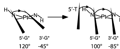
Figure 9. Change in canting when a 5'-T is present relative to the ( R,S,S,R )-BipPt(d(G*pG*)) complex. Torsion angles are provided for the bases in the R-canted starting structure (left) and the low-canted final structure (right). Because the angles are defined with the cis -N, a clockwise rotation causes the 5'-G* value to decrease and the 3'-G* absolute value to increase. The NH groups of the ( R,S,S,R )-Bip ligand are shown.
